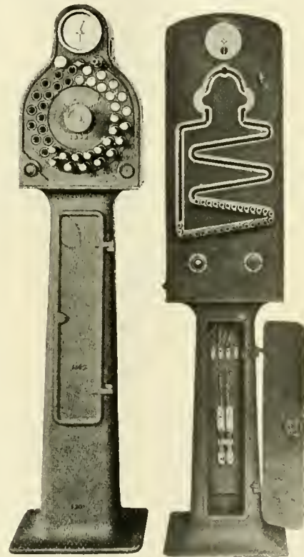
ORIGINAL STAFF MACHINE.
